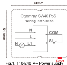
Fig.1. 110-240 V~ Power supply
