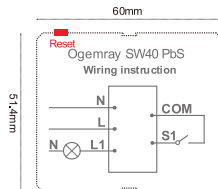
Fig.1. 110-240 V~ Power supply
