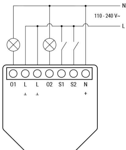
Dual-channel switch mode, AC power supply
